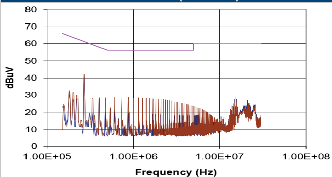
MGJ1D241503SC (Quasi-Peak)
