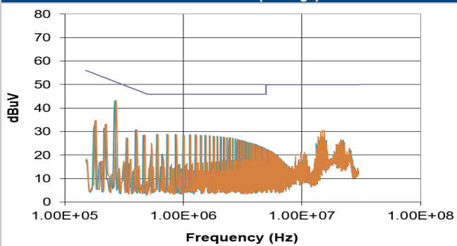
MGJ1D152005SC (Average)
