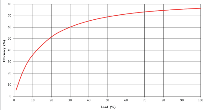
MGJ1D050603SC
