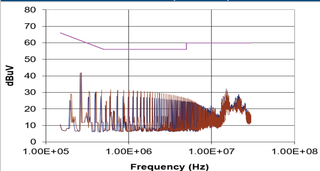
MGJ1D151509SC (Quasi-Peak)
