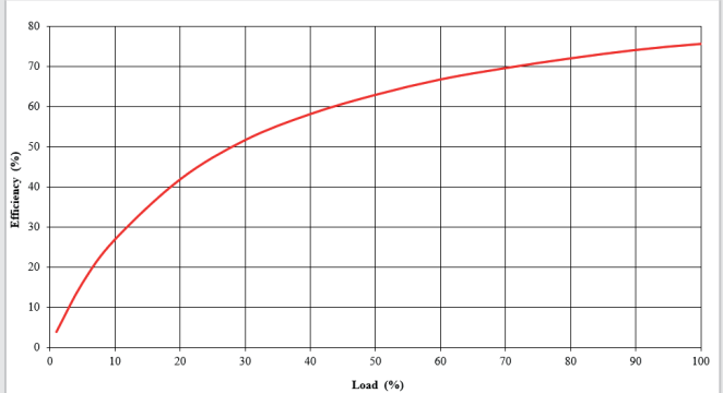
MGJ1D241503SC
