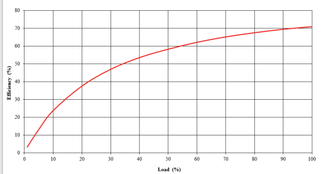
MGJ1D052005SC
