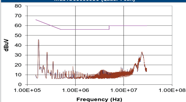
MGJ1D052005SC (Quasi-Peak)
