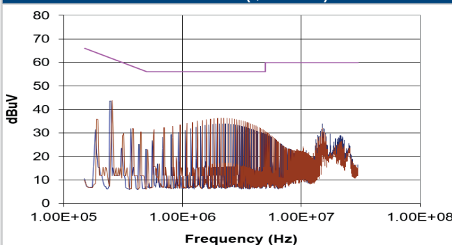
MGJ1D052005SC (Quasi-Peak)
