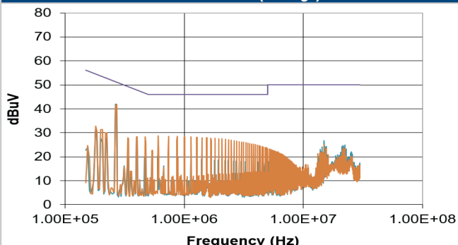
MGJ1D241503SC (Average)
