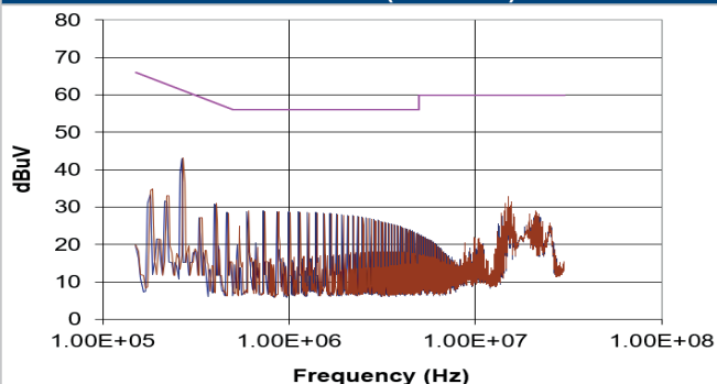
MGJ1D152005SC (Quasi-Peak)
