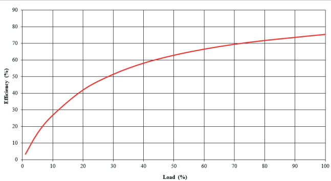
MGJ1D241505SC
