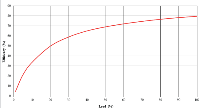
MGJ1D121505SC
