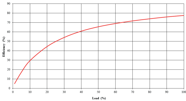
MGJ1D122005SC
