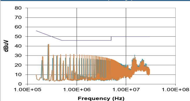
MGJ1D151509SC (Average)
