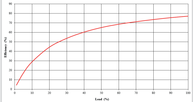
MGJ1D151509SC
